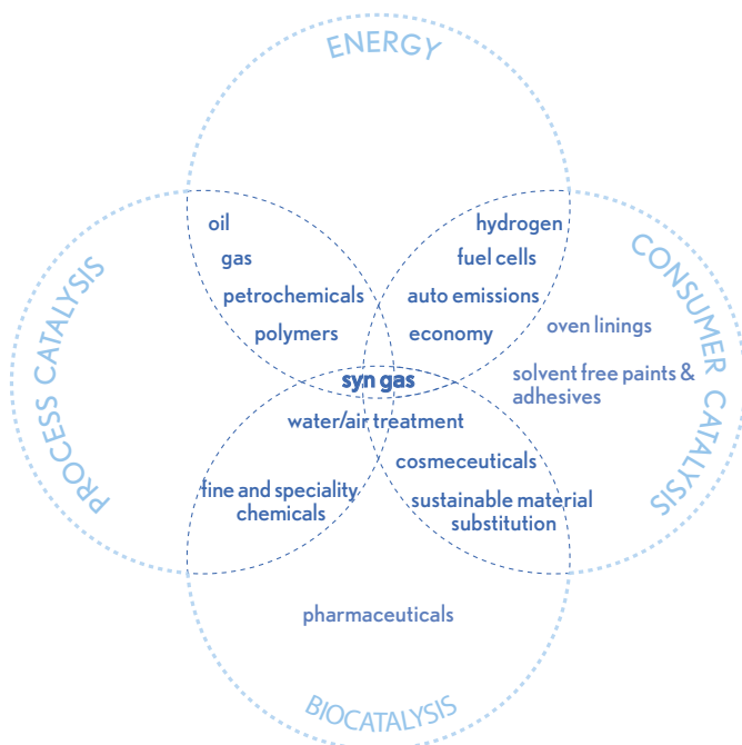
Figure 2.2: Catalysis - one of chemistry's most important and powerful technologies.
