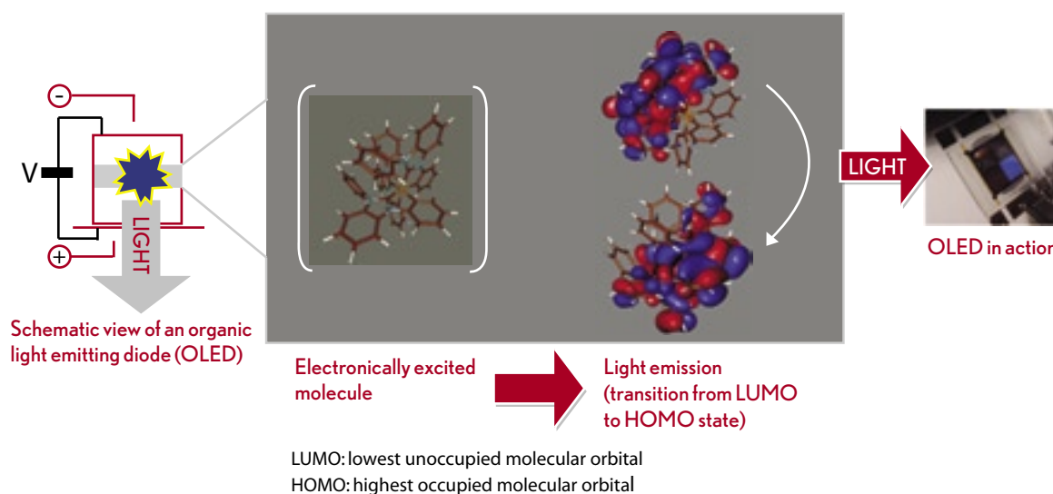
Figure 6.3: Computational material science in the development of a blue OLED: Simulation of emission characteristics.
