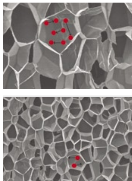
Figure 2.3: By shrinking the cell dimensions within the foam to within the scale of the mean free path of the gas molecules (< 100 nm) the gas based thermal conductivity becomes negligible 9 .
