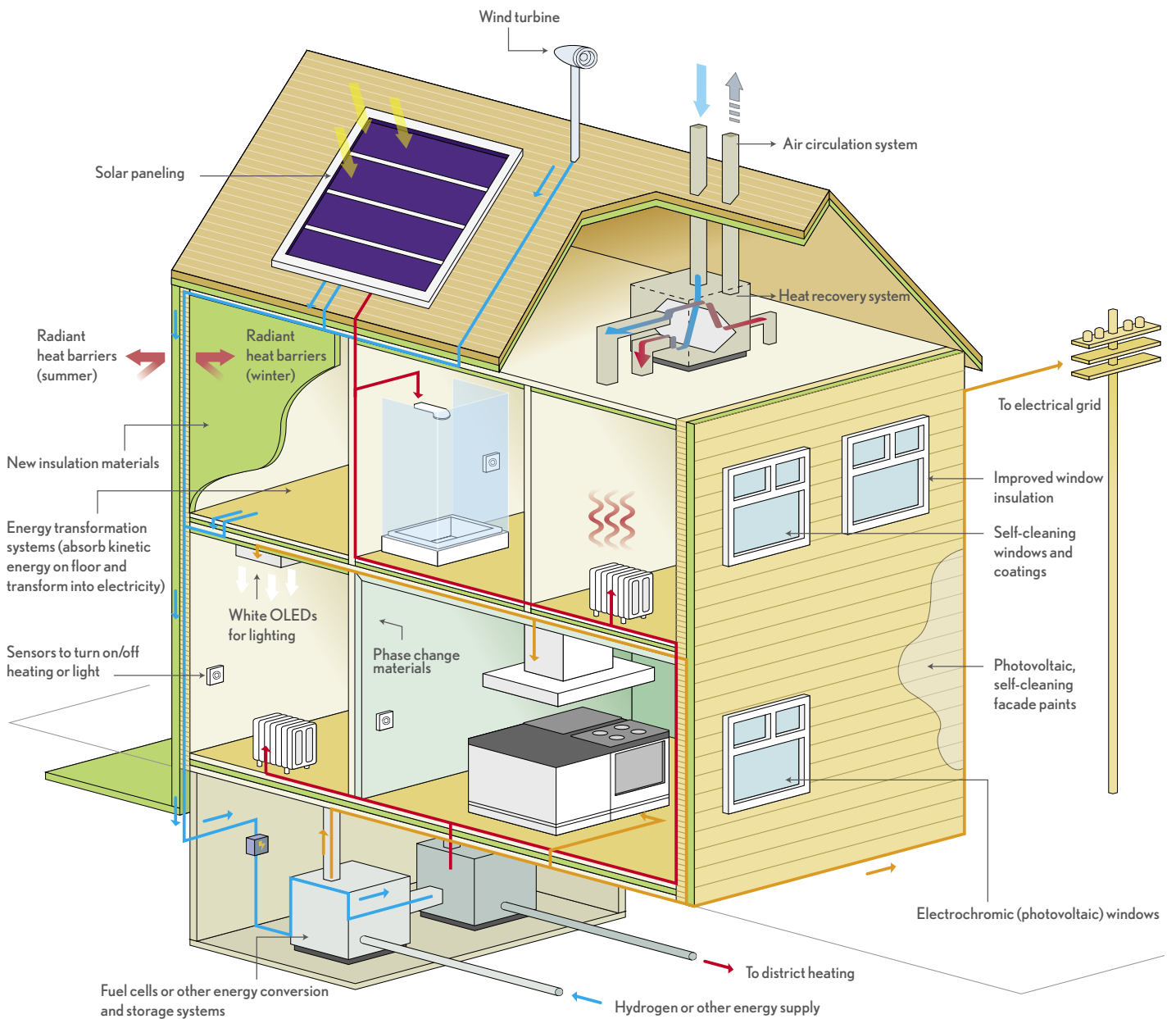
Figure 3.4: The energy-generating home.
