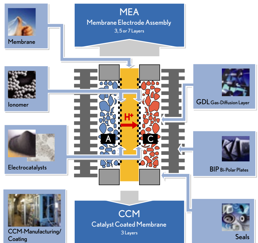
Figure 2.6: The components, materials and productions technologies necessary to construct a single cell of a fuel cell stack.
